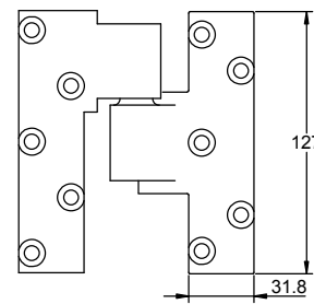
ML19 intermediate pivot
